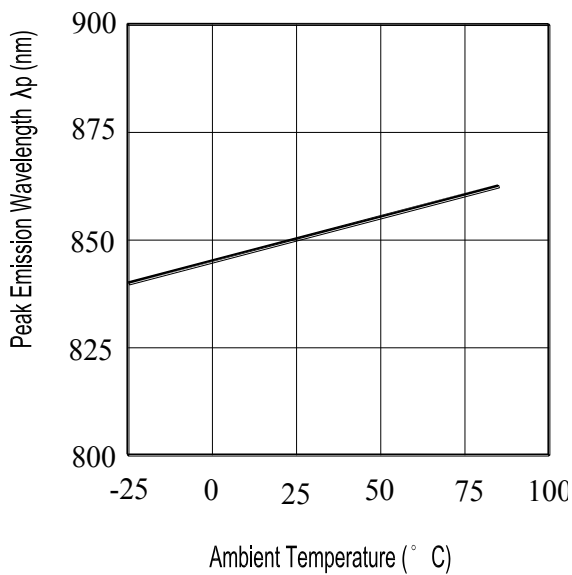
Fig.3 Peak Emission Wavelength λp vs. Ambient Temperature
