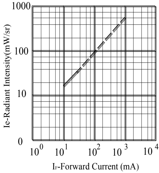
Radiant Intensity vs. Forward Current
