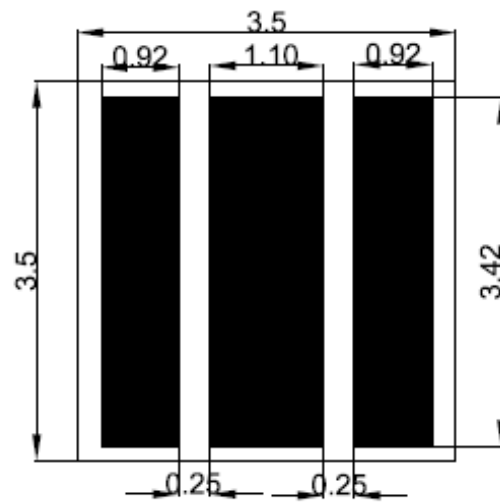
Soldering patterns
