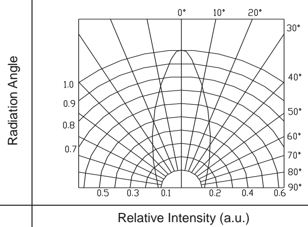
Directivity (Ta=25°C)
