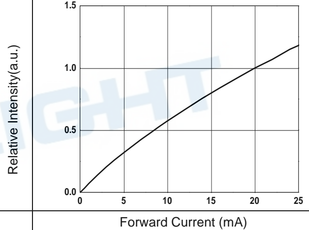
Relative Intensity vs. Forward Current (Ta=25°C)
