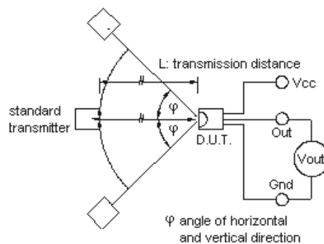
Fig.3 Measuring System
