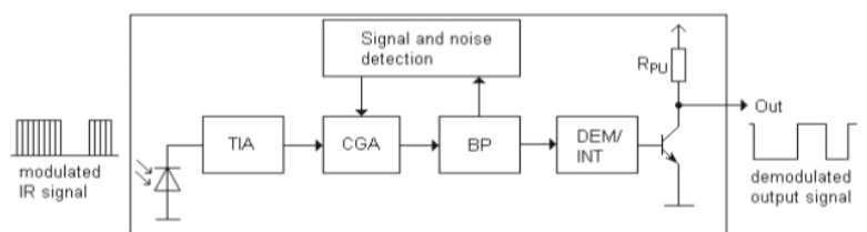
Fig.1 Block Diagram
