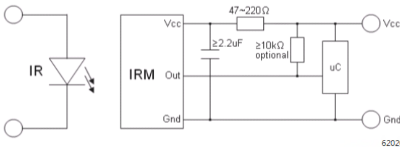
Fig.9: application circuit
