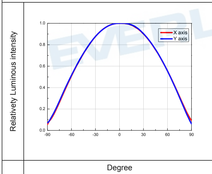
Typical Radiation Patterns
