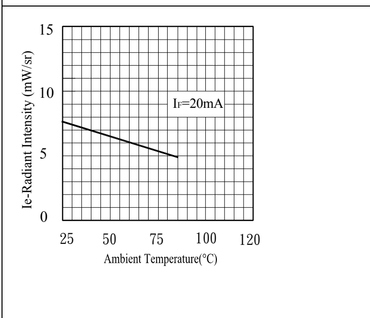
Relative Intensity vs. Ambient Temperature(°C)
