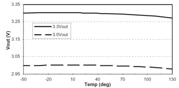
Fig. 15: V_{OUT} vs. Temp (adjustable)
