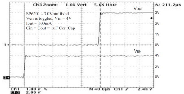
Fig. 23: Turn on time, I_O=100\text{mA} , 4V_{IN}
