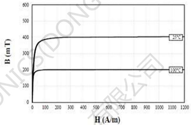
Saturation Flux Density V.S. Magnetic Field
