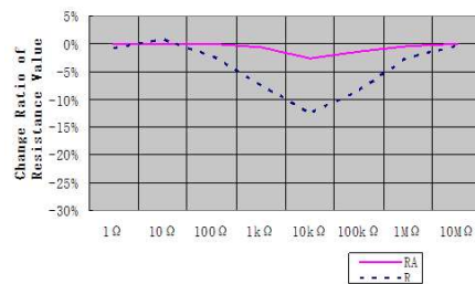
2010size: ±8kV
