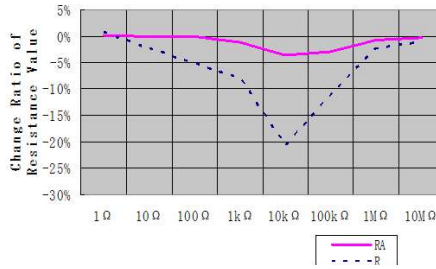
1210size: ±5kV
