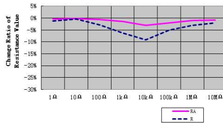
2010size: ±8kV
