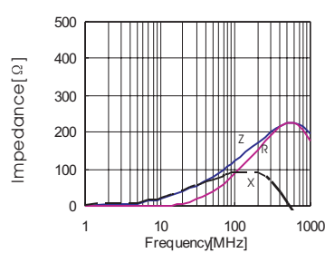
CBM160808U121T
