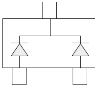
COMMON CATHODE
