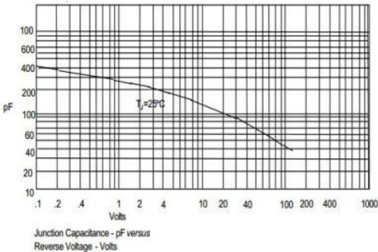
FIG.4-TYPICAL JUNCTION CAPACITANCE
