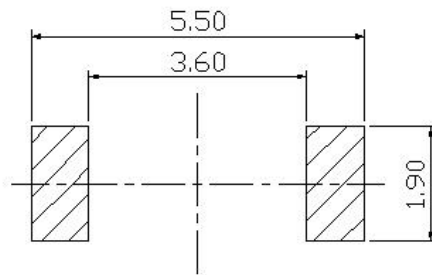
Printed Circuit board dimensions
