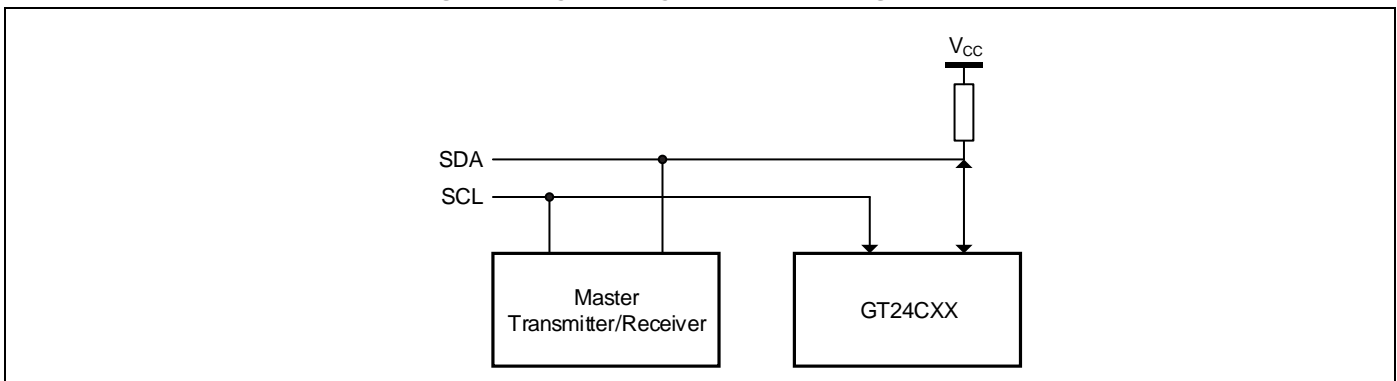
Figure 1. Typical System Bus Configuration
