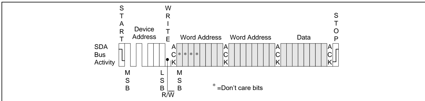
Figure 8. Byte Write
