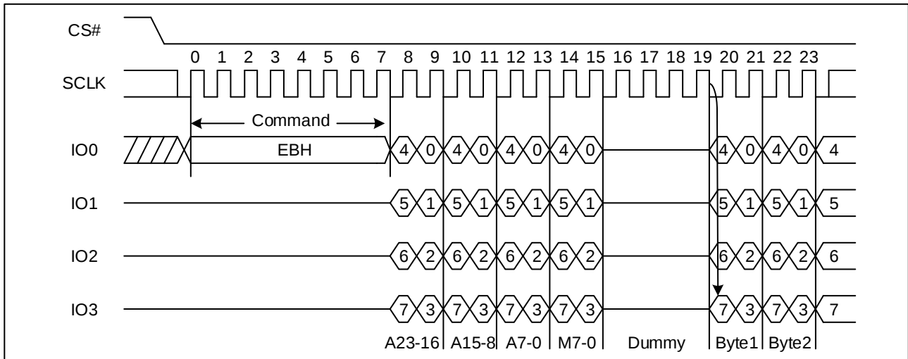
Figure 13. Quad I/O Fast Read Sequence Diagram ((M5-4) \neq (1, 0))
