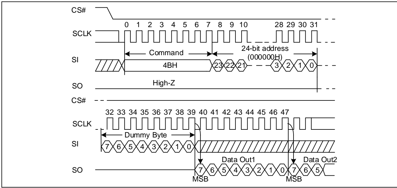
Figure 22. Read Unique ID Sequence Diagram
