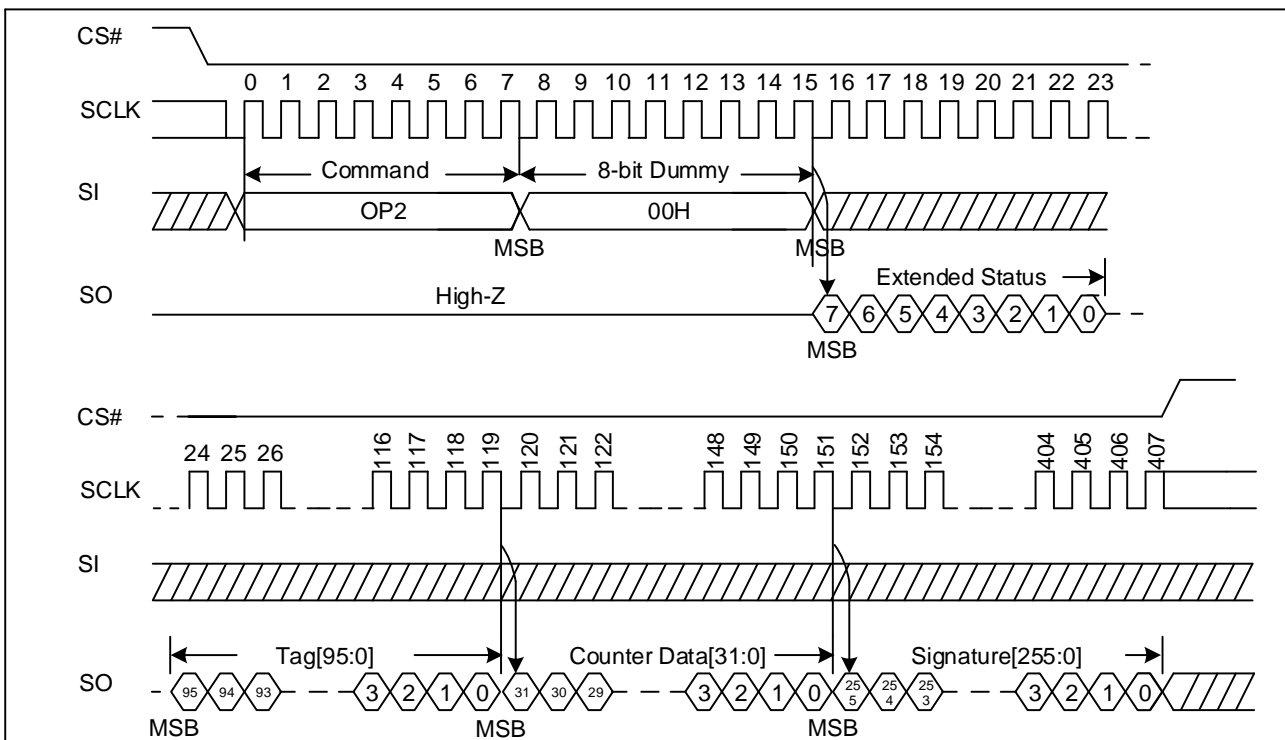
Figure 37. Read Data Sequence Diagram
