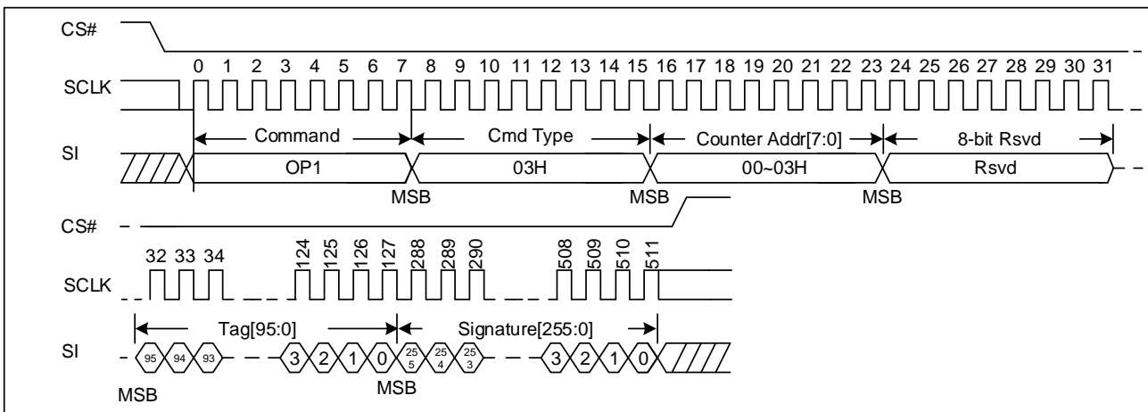
Figure 36. Request Monotonic Counter Sequence Diagram
