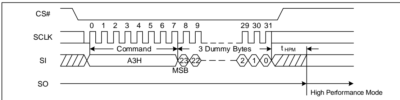
Figure 19. High Performance Mode Sequence Diagram
