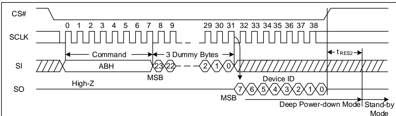
Figure 31. Release Power-Down/Read Device ID Sequence Diagram
