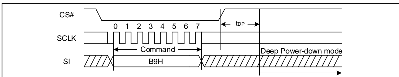
Figure 29. Deep Power-Down Sequence Diagram
