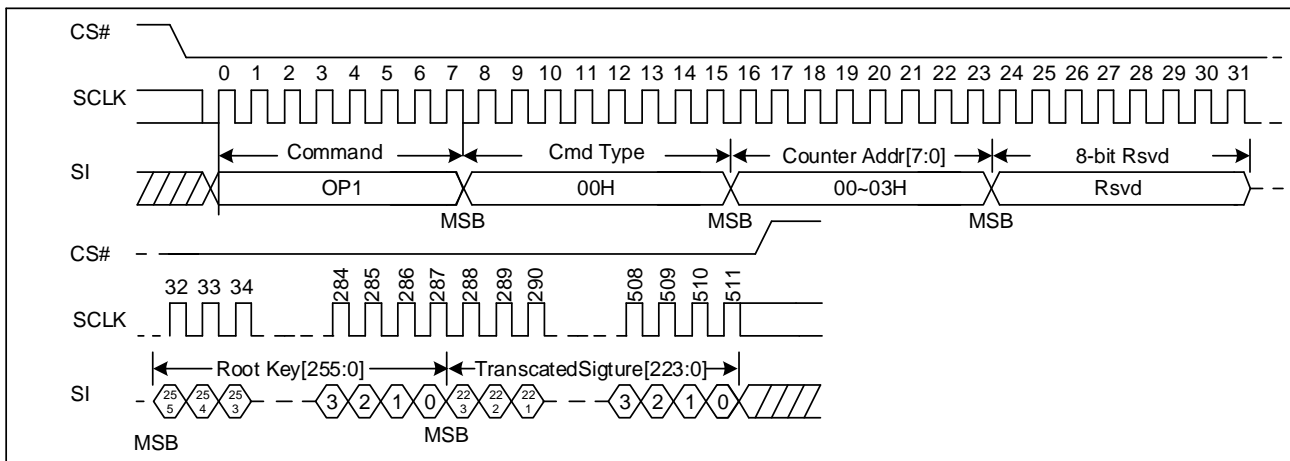
Figure 33. Write Root Key Register Sequence Diagram
