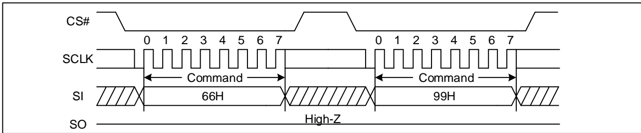
Figure 26. Enable Reset and Reset command Sequence Diagram
