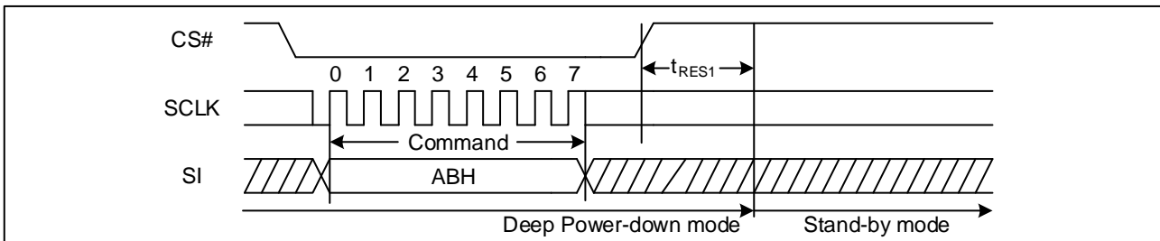
Figure 30. Release Power-Down Sequence Diagram
