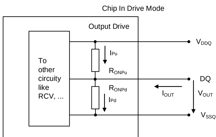
Figure 8-1. Output Driver
