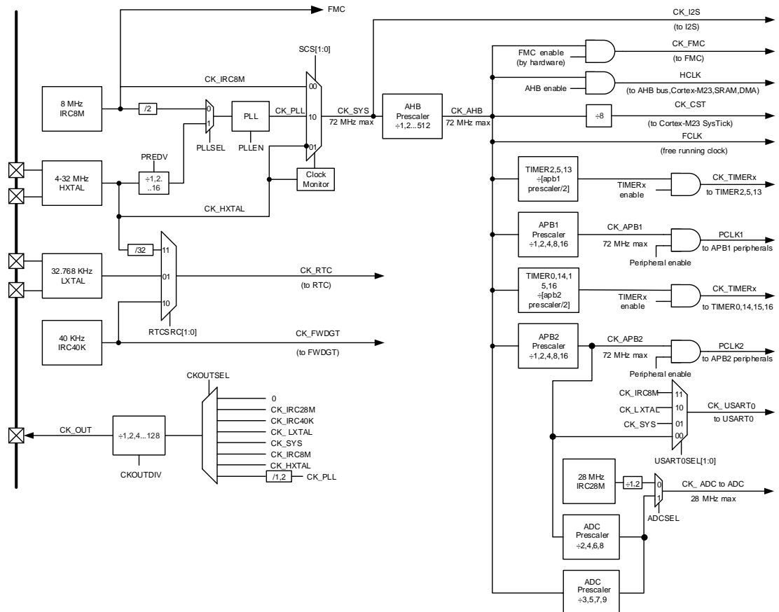
Figure 2-7. GD32E230xx clock tree
