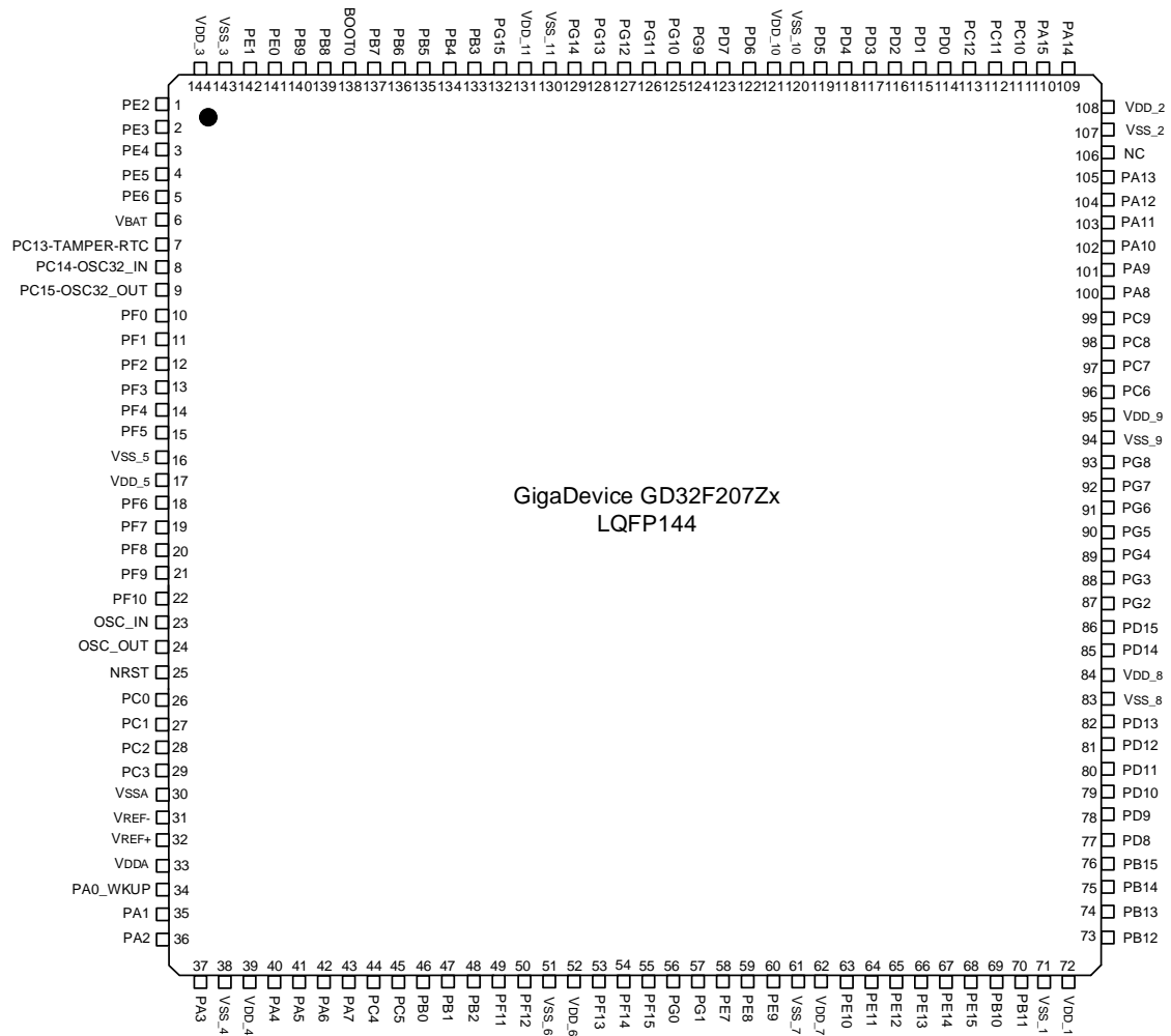
Figure 3. GD32F207Zx LQFP144 pinouts
