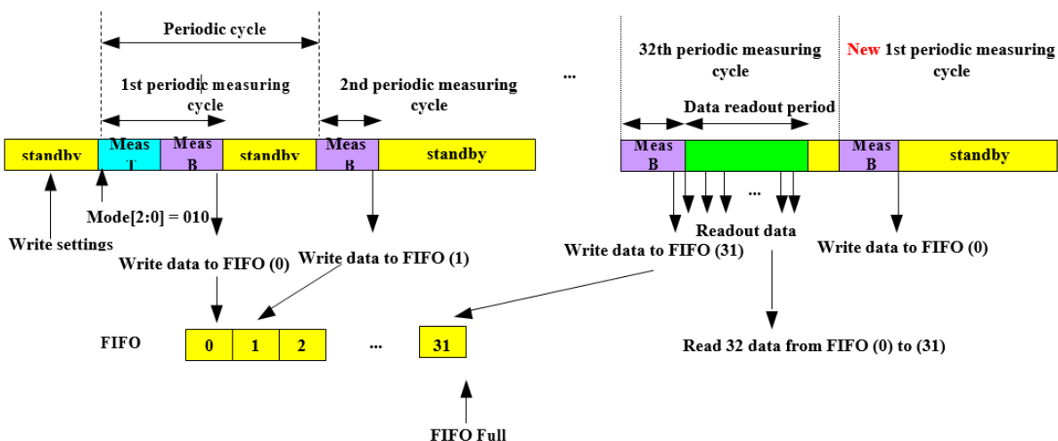
Figure 2: FIFO stream mode
