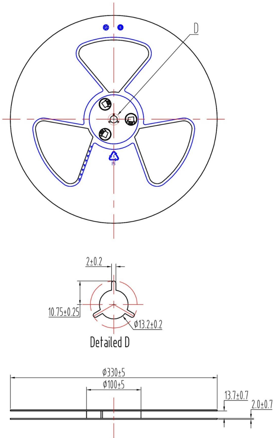
Figure 9: Carrier Tape (2)
