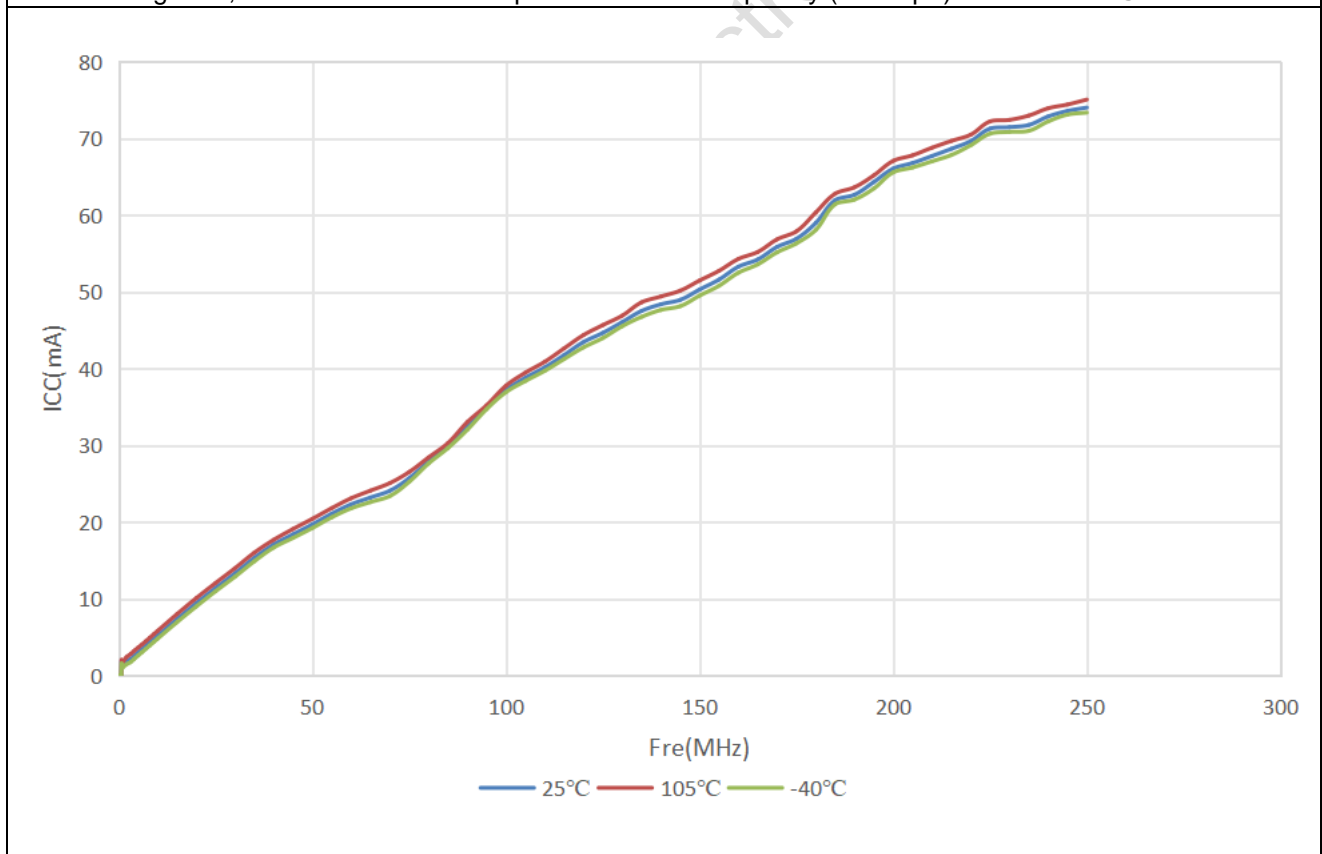
Figure 5, Device Power Consumption vs. Clock Frequency ( C_L = 5pF ) of GM51104 @VDD=3.3V
