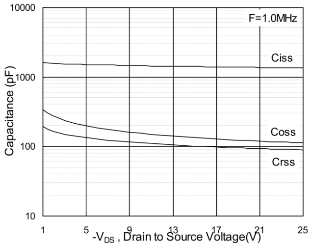
Fig.7 Capacitance
