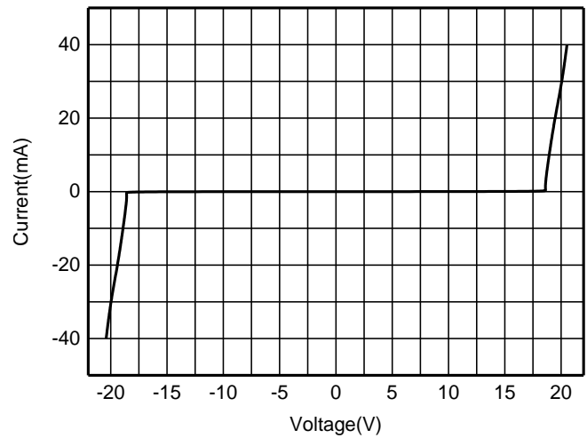
I-V Curve
