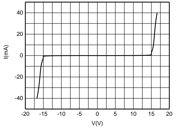
I-V Curve
