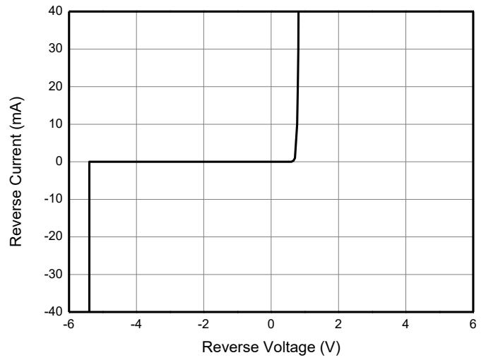
I-V Curve
