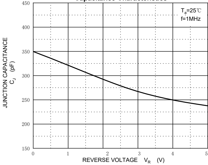
Capacitance Characteristics
