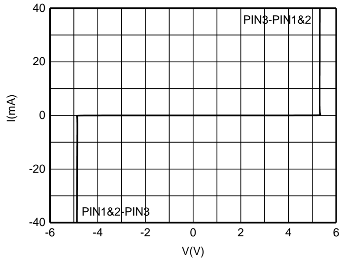
I-V Curve
