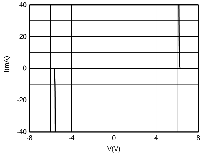
I-V Curve
