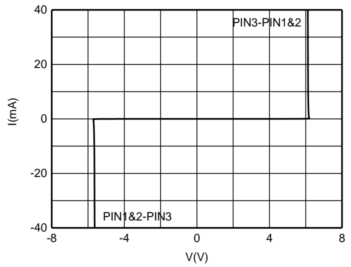
I-V Curve
