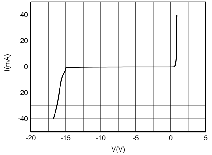
I-V Curve
