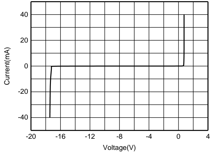
I-V Curve
