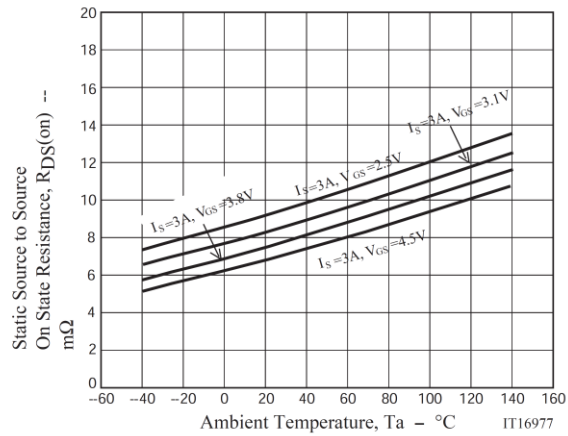
CJCD2004 R_{DS(on)} vs. T_A
