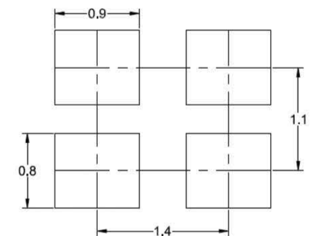
Recommended Land Pattern Tolerance: ±0.1
