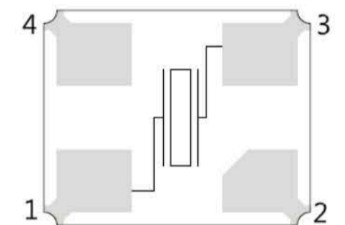
Internal Connection (Top View)
