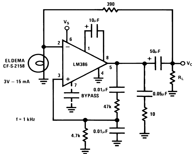
Low Distortion Power Wienbridge Oscillato
