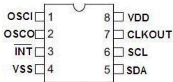
SOP-8/MSOP-8/DIP-8
