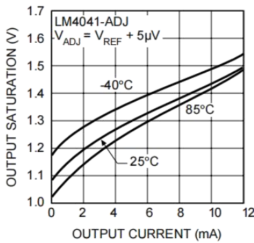
Output Saturation
