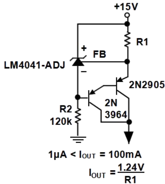
Figure 10. Current Source
