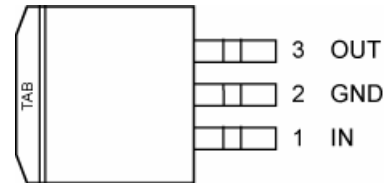
3-Pin TO-263 (D²Pak) (UT) MIC29150/29300
