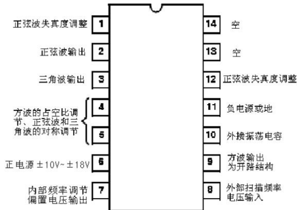
DIP-14/SOP-14/TSSOP-14
