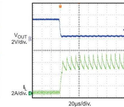
Short Circuit Test Waveforms
