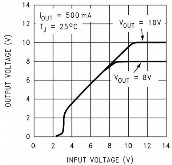
Figure 14. Low-Voltage Behavior
