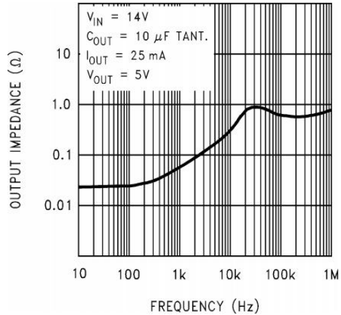
Figure 10. Output Impedance
