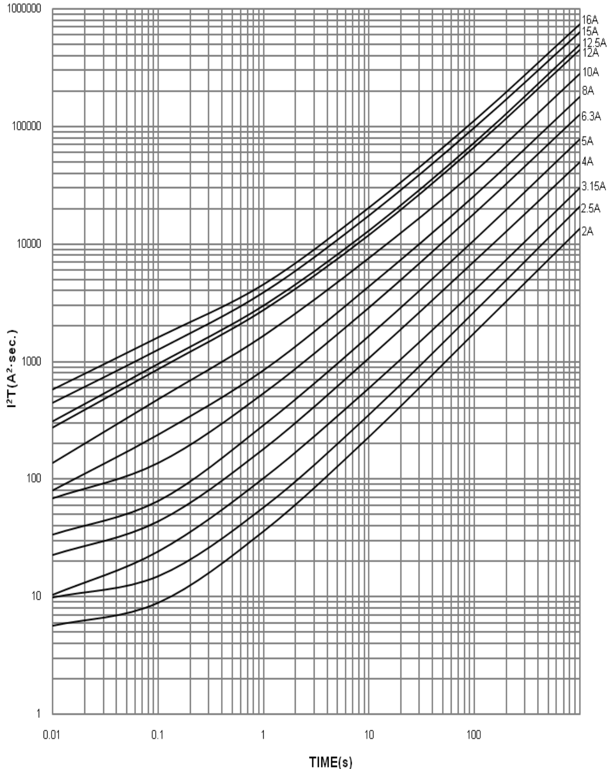
5HT(P) RoHS Average I 2 T-T Characteristics Curve(For Reference Only)
