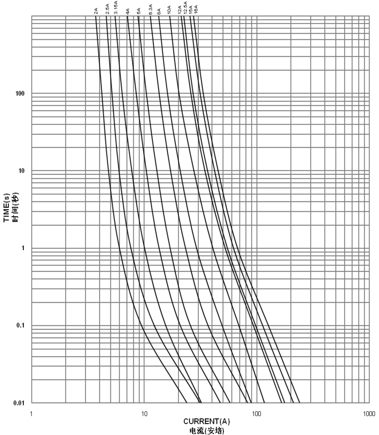
5HT(P) RoHS Average I-T Characteristics Curve(For Reference Only) 5HT(P) RoHS 平均电流-时间曲线图(仅供参考)
