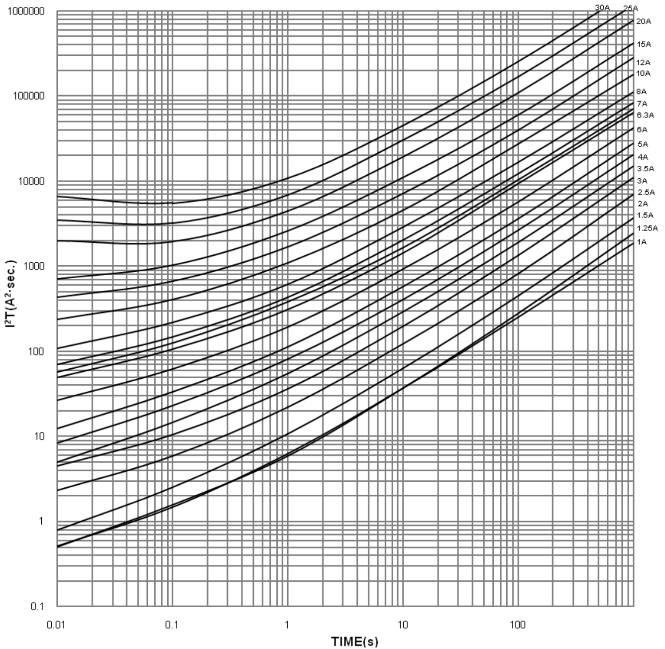
65TS RoHS Average I 2 T-T Characteristics Curve(For Reference Only)
