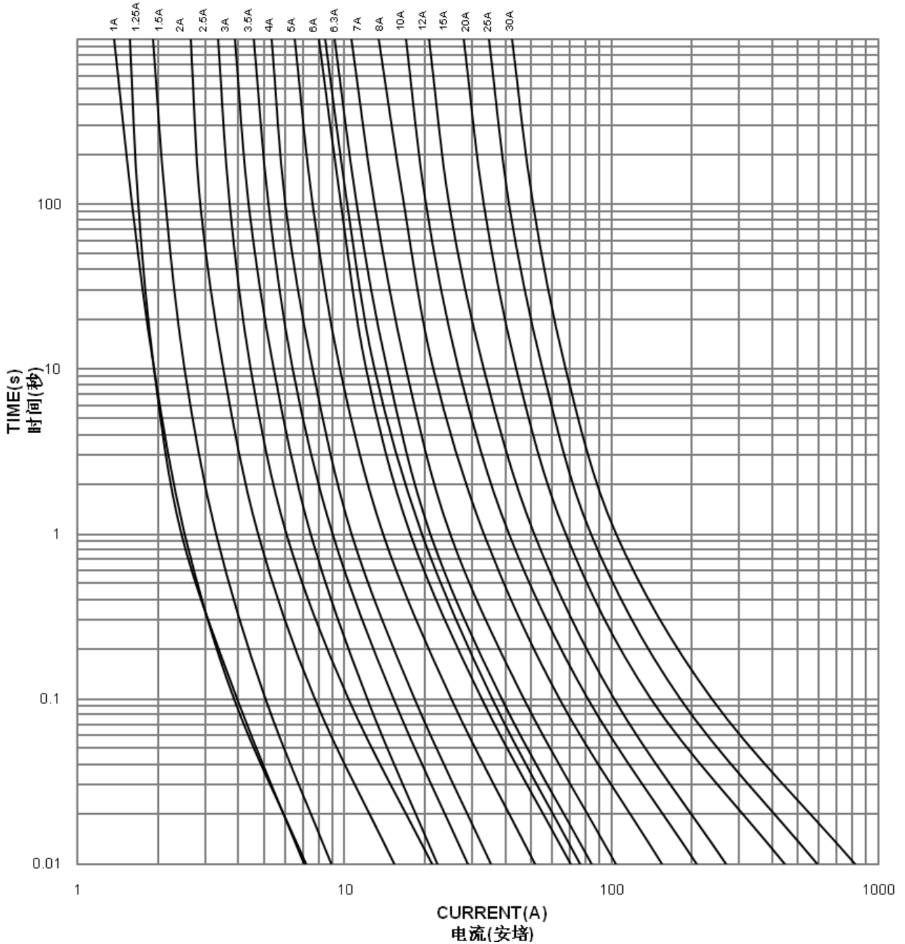
65TS AVERAGE I-T CHARACTERISTICS CURVE(FOR REFERENCE ONLY) 65TS 平均I-T曲线图(仅供参考)
