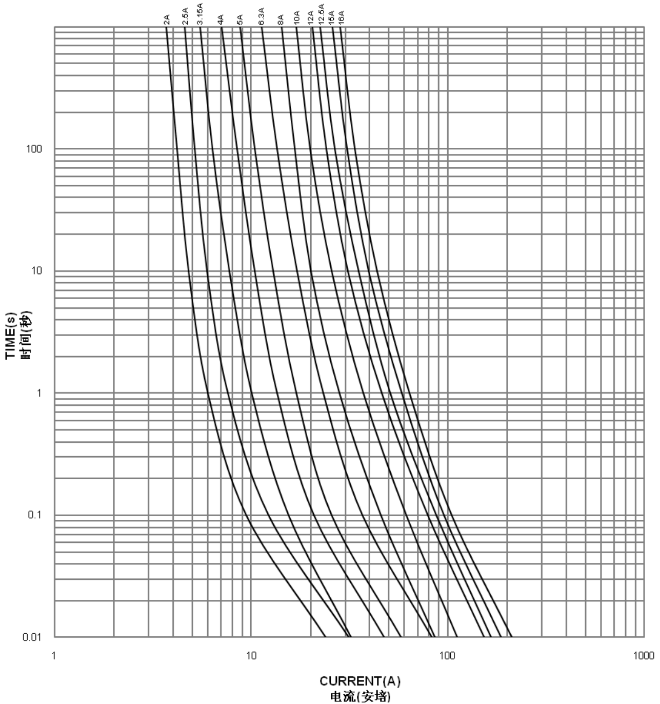
5HT RoHS Average I-T Characteristics Curve(For Reference Only) 5HT RoHS 平均电流-时间曲线图(仅供参考)
