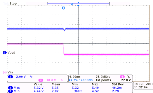
线性瞬态响应：HT7350-1 ( I_{OUT}=10mA )
