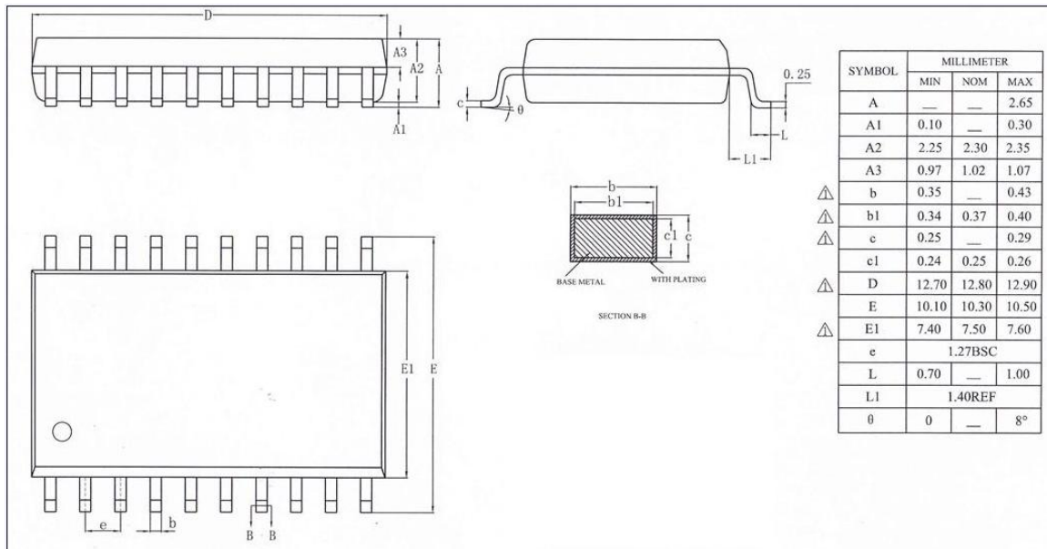
Figure 21-1 SOP20 封装尺寸
