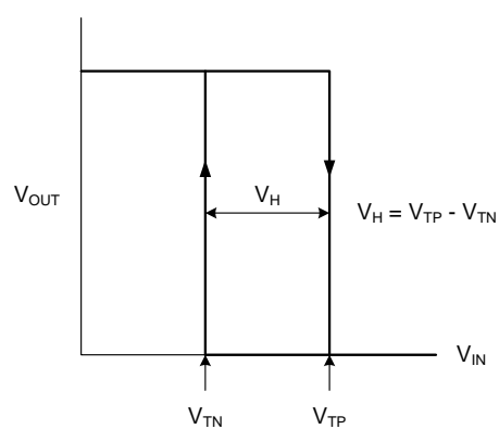
Fig. 2. Hysteresis Characteristic
