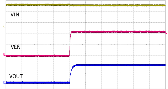
VIN : 2.0V/div, VEN : 2.0V/div, VOUT : 2.0V/div, Time : 5ms/div Start Up by External VEN @ Iout=1A
