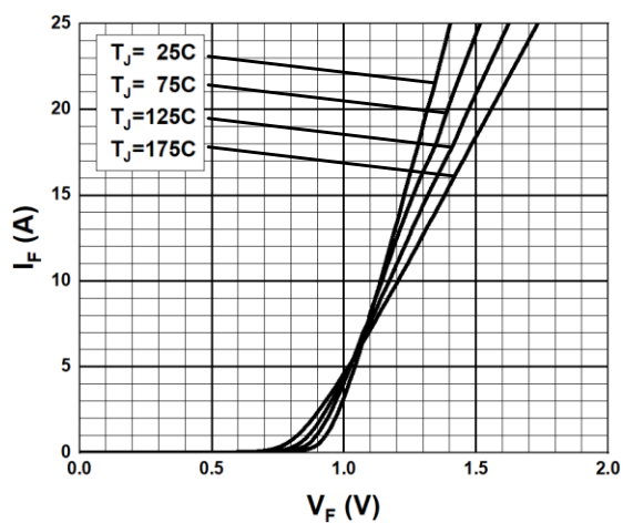
Fig. 1 Forward Characteristics
