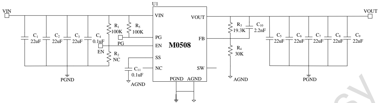
Figure 2. Typical Application Circuits of M0508 for 1V Output
