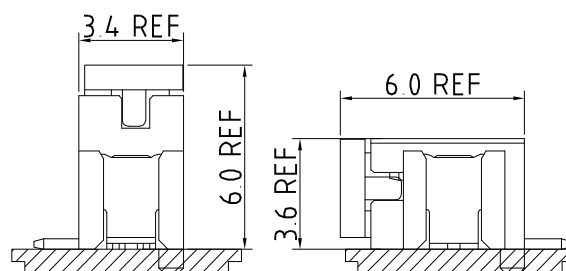
Vertical SMT Type Right Angle SMT Type
